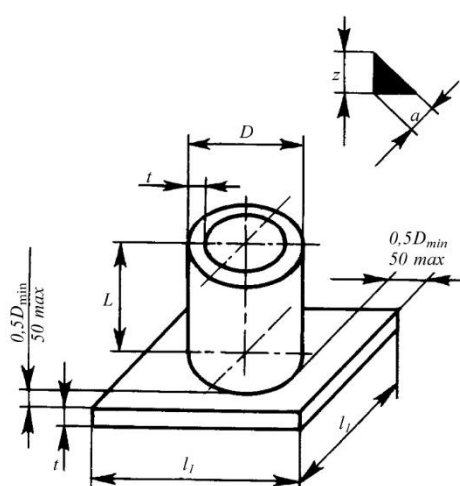
Fig. 4 Test piece of P 4 fillet-welded pipe joint
