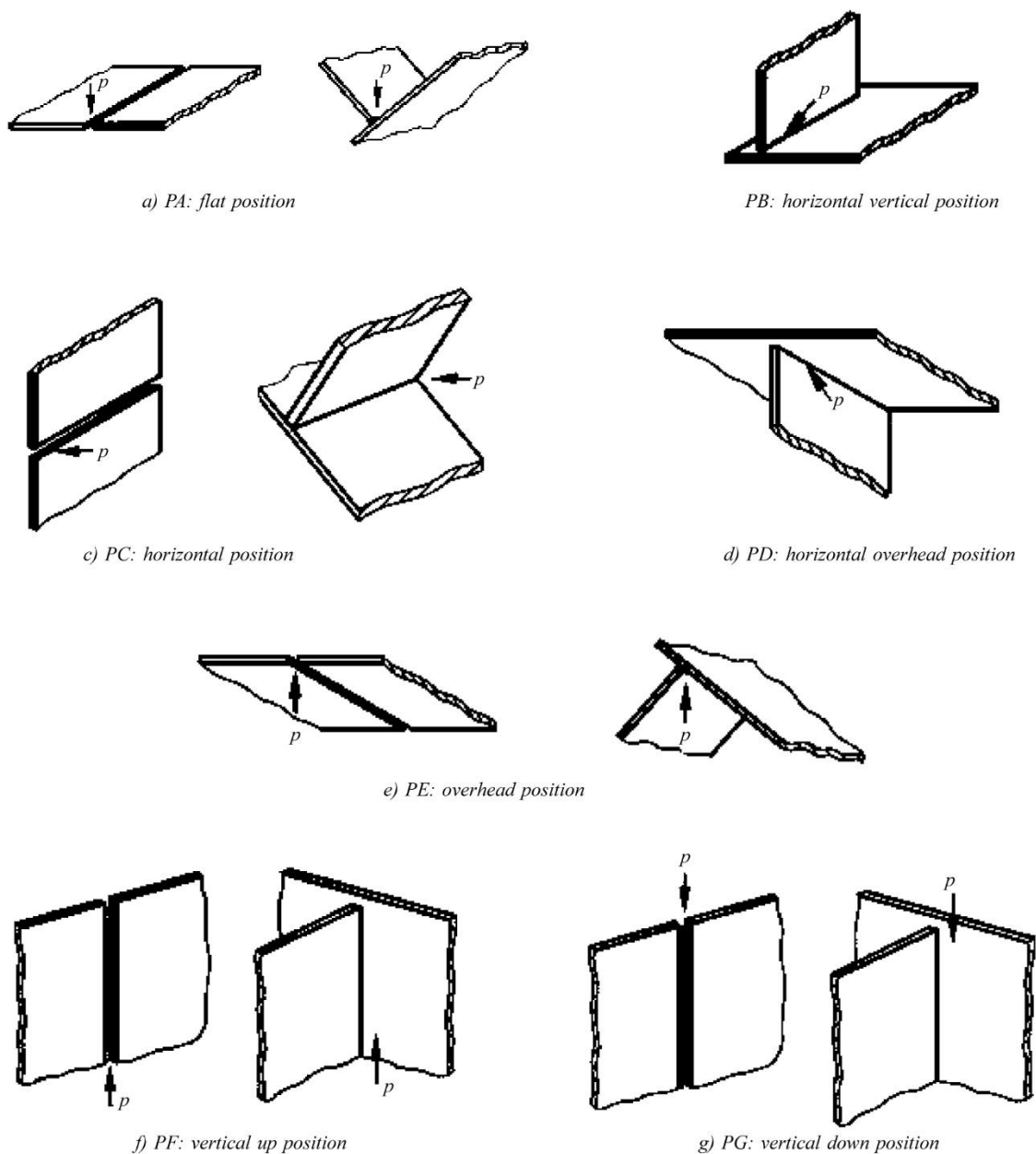
Fig. 1 Welding positions for plates
