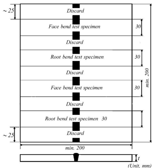
Fig. 1.1 Dimensions and types of test piece for butt welds ( T < 12 mm)
