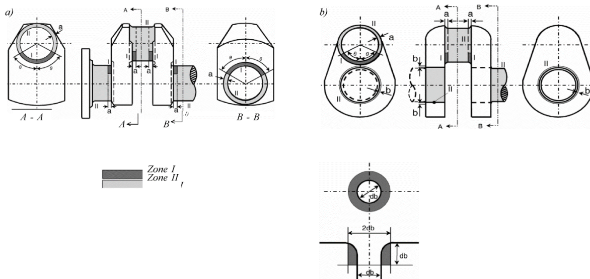
Fig. 2.5.2.3.3-1 Zones for magnetic particle/dye penetrant testing on crankshafts:
